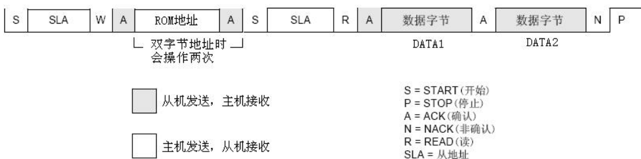
USB-I2C Adapter I2C Read Timing
