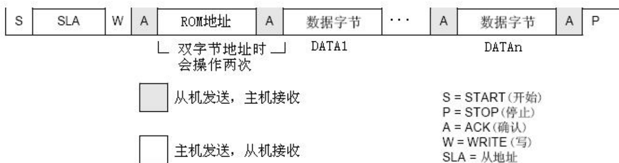
USB-I2C Adapter I2C Write Timing
